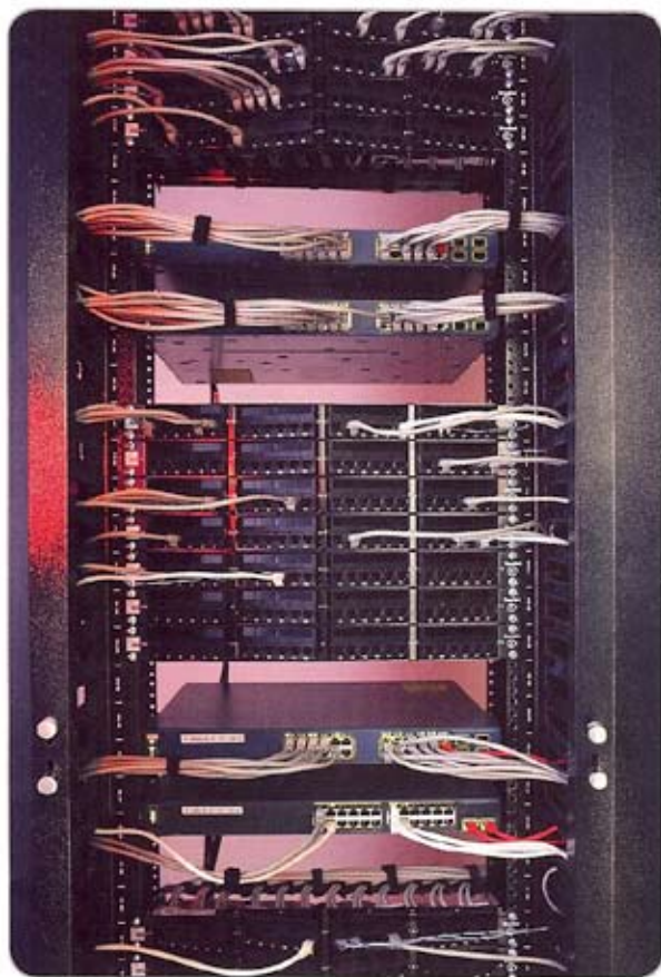
24-port Dynamic Angle Patch Panels direct the patch cords toward cable management on the sides of the rack.
